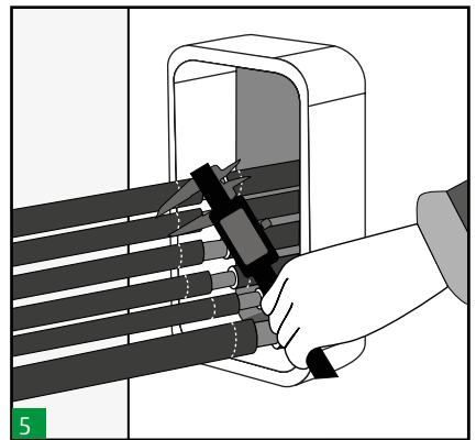
5 Take measures of cables diameters and select the appropriate Hawke tolerant blocks.
