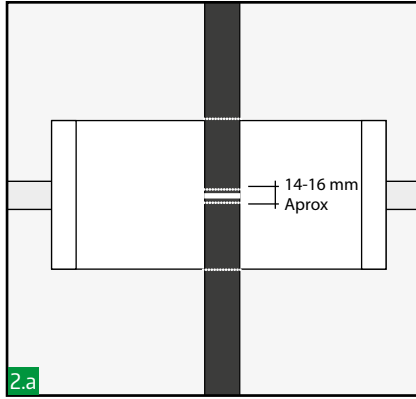
2.a Mark each cable in the centre of the frame and 7-8mm either side of this point. Also, recommendable to mark the cable in both ends of the frame. EMC marking tool could help you to reduce time and ensure a correct marking.
