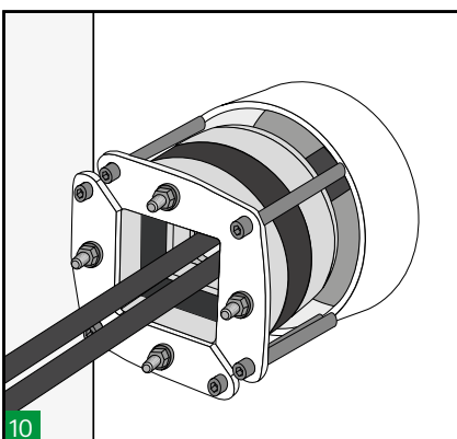
Extraction is achieved by releasing the compression, i.e. by reversing steps 7 and 8 and screwing M8 bolts (not supplied) into the threaded holes at each corner of the front plates. These releases the assembly from the aperture and allows the system to be disassembled.
