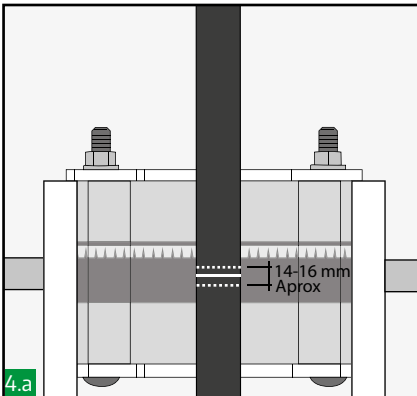
4.a Mark each cable in the centre of the frame and 7-8mm either side of this point. Also, recommendable to mark the cable in both ends of the frame.
