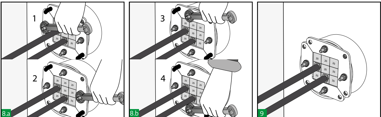
Tighten the nuts approximately 2mm each time following alternate tightening sequence, applying equal pressure to both plates. A minimum of 10 mm of thread should protrude on each bolt. Use a ratchet spanner for an easier installation.
