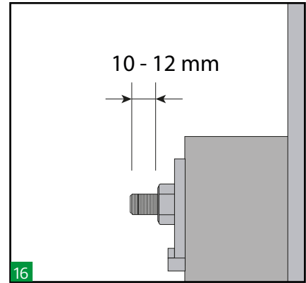
16 Approximately 10-12 mm of thread should protrude on each bolt to ensure the sealing.
