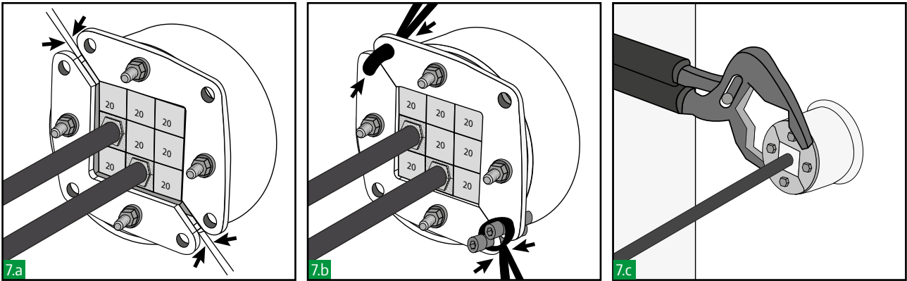
Slide the two front plates together and keep it fixed. Ensure all the blocks are located inside the front retaining lip. For an easier installation, cable ties, bolts or adjustable pliers can be used to close this plates.
