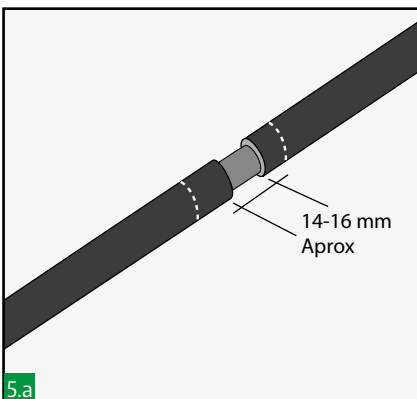
5.a Cut and remove cable sheath between two central marks, to expose the cables conductive screen.
