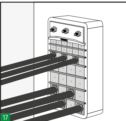
17 Make a visual inspection of the transit. Check that marks in all the cables are visible to guarantee blocks and cable copper tapes are aligned.
