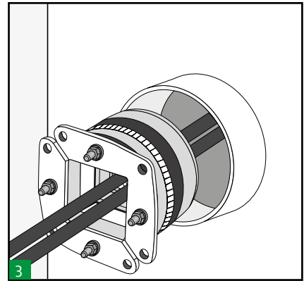
3 Insert the round transit frame completely in the sleeve around the cables and open the two front plates. (HRTO30,HRTO40&HRTO50 front plates are fixed). No lubricant should be applied to the aperture or outside of the frame.
